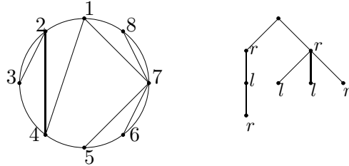
Figure 2: Two representations of a noncrossing tree
