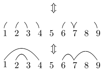
Figure 2.3: A pair of noncrossing free Dyck paths and the corresponding partition.
