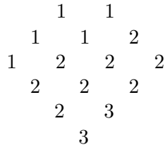
Figure 2.1: A triple of noncrossing free Dyck paths and the corresponding plane partition.
