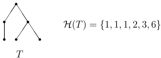
Figure 1: The multi-set of hook lengths of a tree.
