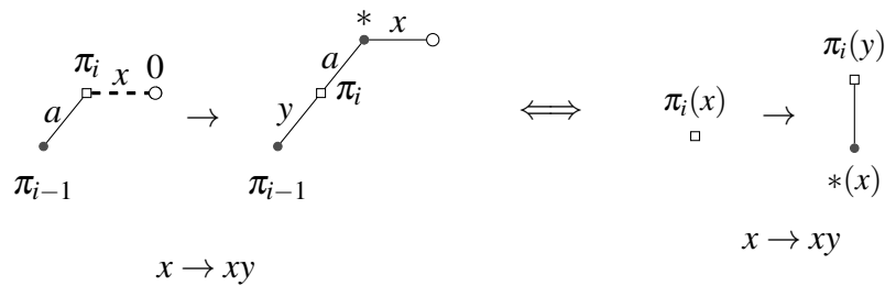
Figure 13: The case k = i + 1 and \pi_{i-1} < \pi_i .
