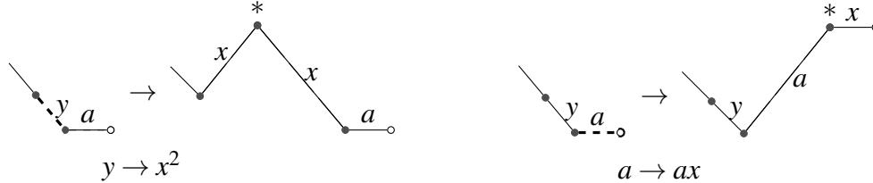
Figure 4: The labeling of \sigma ends with ya .
