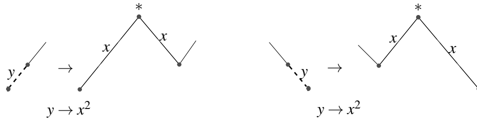
Figure 2: Insertion at a position labeled by y .
